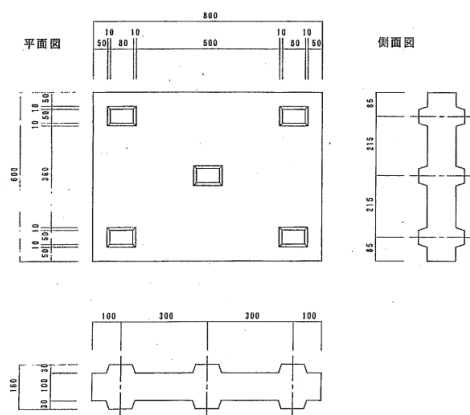
平板礁 800x600x100/30-30
