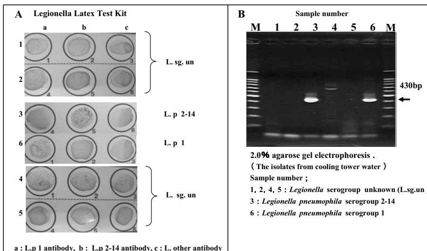
Fig. 3. Result of serotyping (A) and single PCR products (B) from Legionella species.
